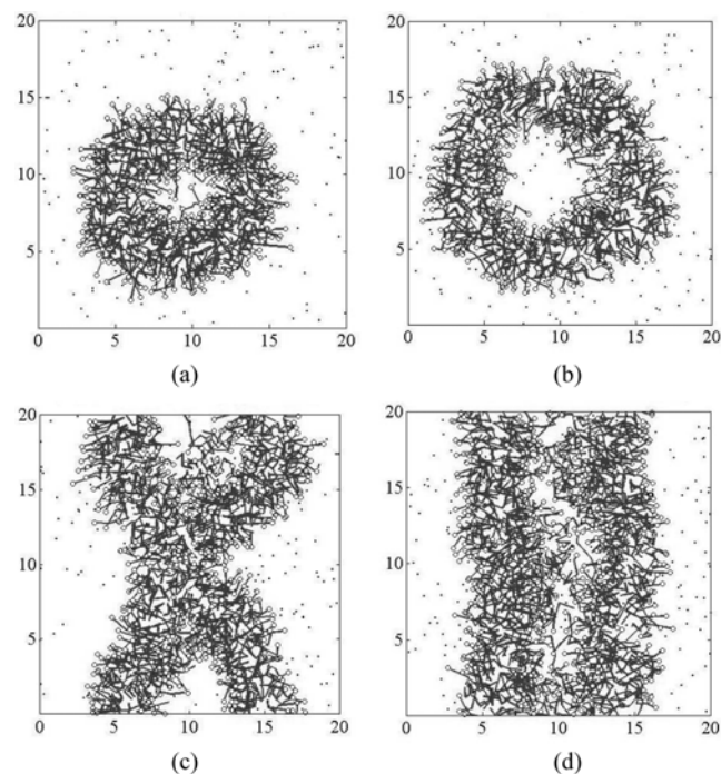
Fig. 3. Slice images of Fig. 2: (a) \phi=0.15 , (b) \phi=0.20 , (c) \phi=0.24 , (d) \phi=0.26 ; the head group ( \circ ), the hydrocarbon chain (—) and the water contained sodium ion ( \bullet ).
